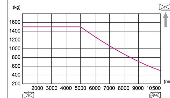
Load Curve
